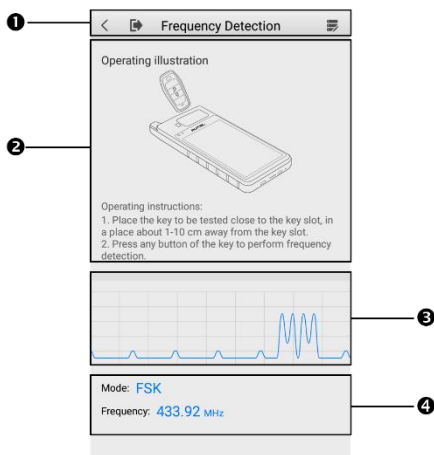
Figure 6-7 Frequency Detection Screen
