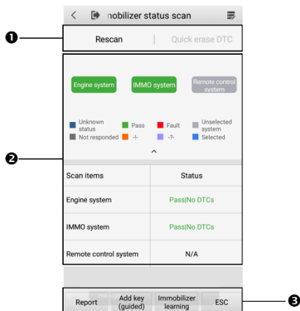
Figure 7-4 IMMO Status Scan
