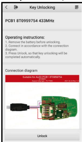
Figure 8-7 Key Unlocking Operation Screen
