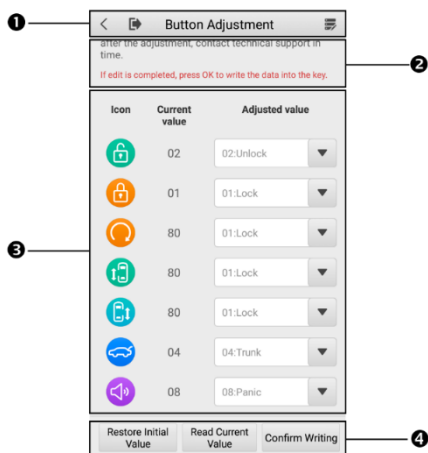
Figure 8-9 Button Customization Screen
